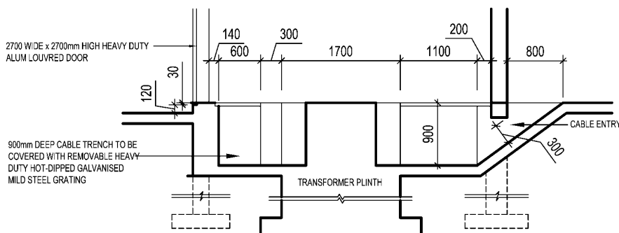
SECTION P-P
