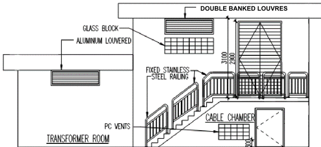
FRONT ELEVATION
