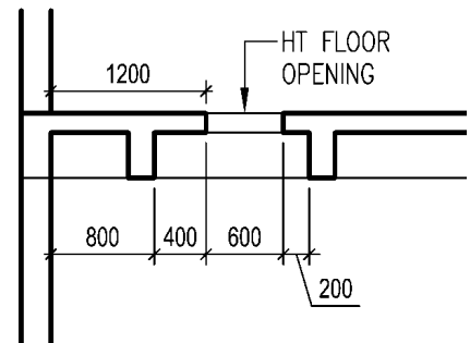
SECTION Q-Q
