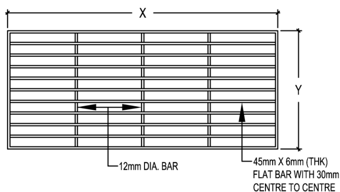
TYPICAL HEAVY DUTY HOT-DIPPED GALVANISED MILD STEEL GRATING DETAIL
