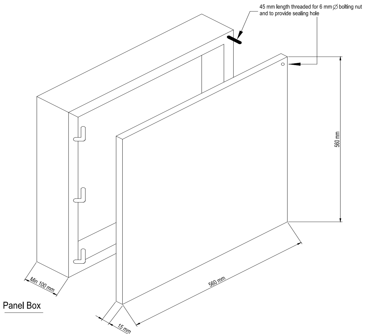
Meter Mounting Panel
